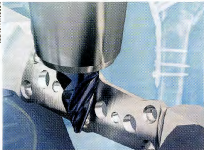
Curvemax curve segment mills can machine a titanium bone plate up to 85 % faster than conventional ball-shaped mills, Inovatools claims.
